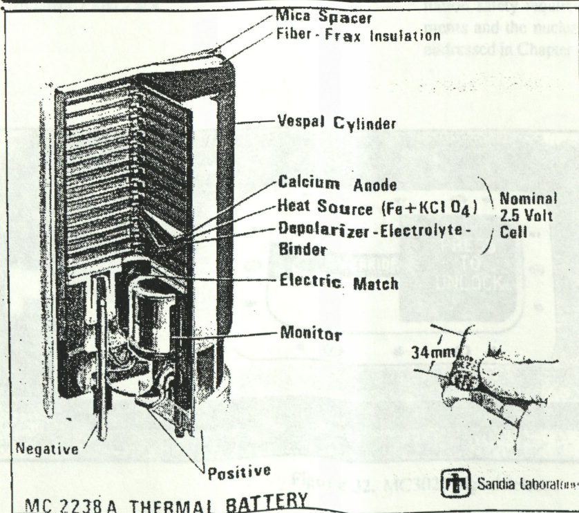
Figure 30. MC2238A Thermal Battery
